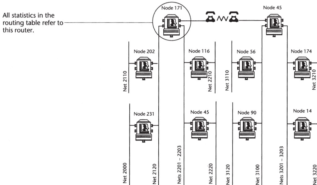
Internetwork with 2 extended cables and 10 nonextended cables, including a dial-up link between the routers at nodes 171 and 45
