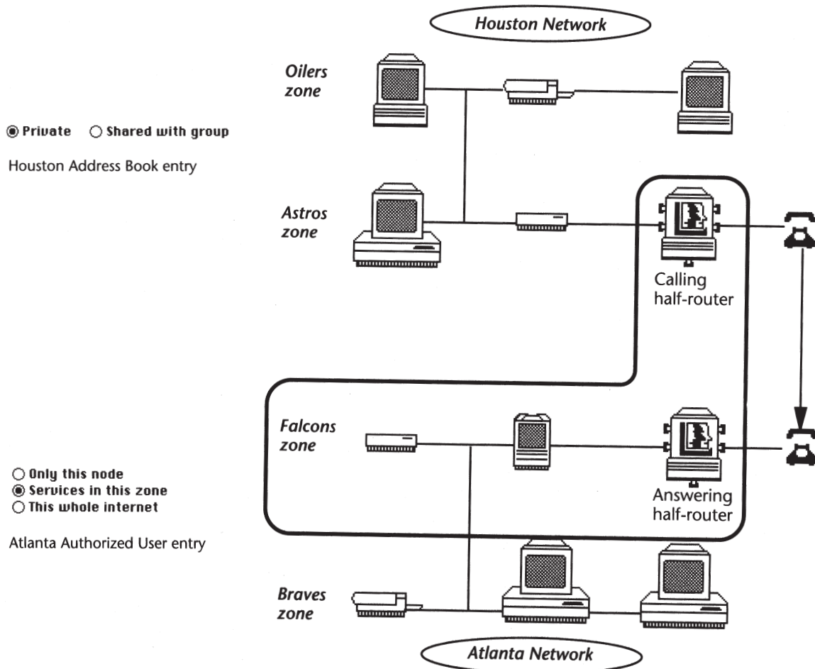
Houston calling Atlanta: Moderate scope connection 1
